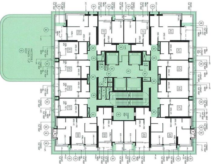
TOWER 1, 2ND FLOOR PLAN
