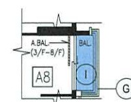
TOWER 1 PART PLAN AT 3rd - 8th FLOOR (FLOOR NO. 4th FLOOR OMITTED)
