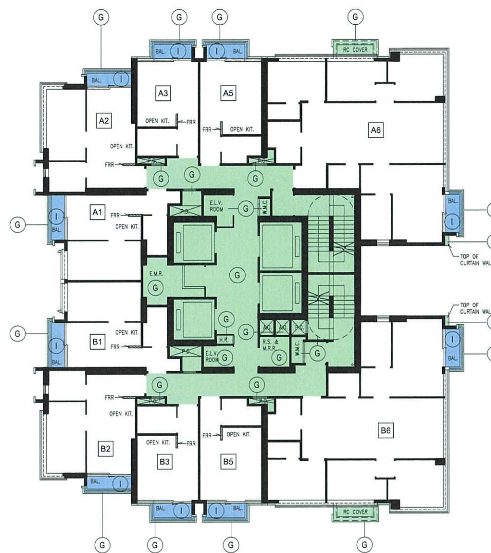
TOWER 1, 38TH FLOOR PLAN
