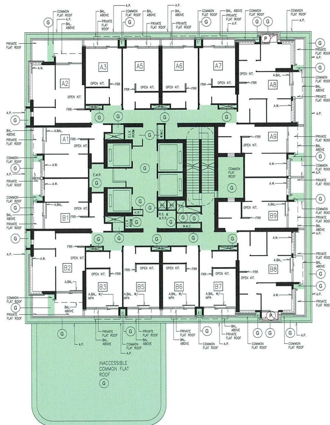
TOWER 1, 2ND FLOOR PLAN
