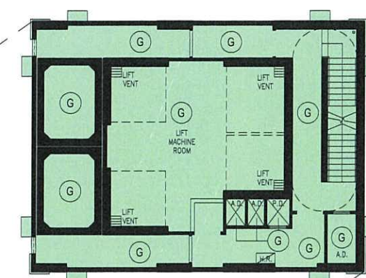
TOWER 1, MECHANICAL 1 FLOOR PLAN
