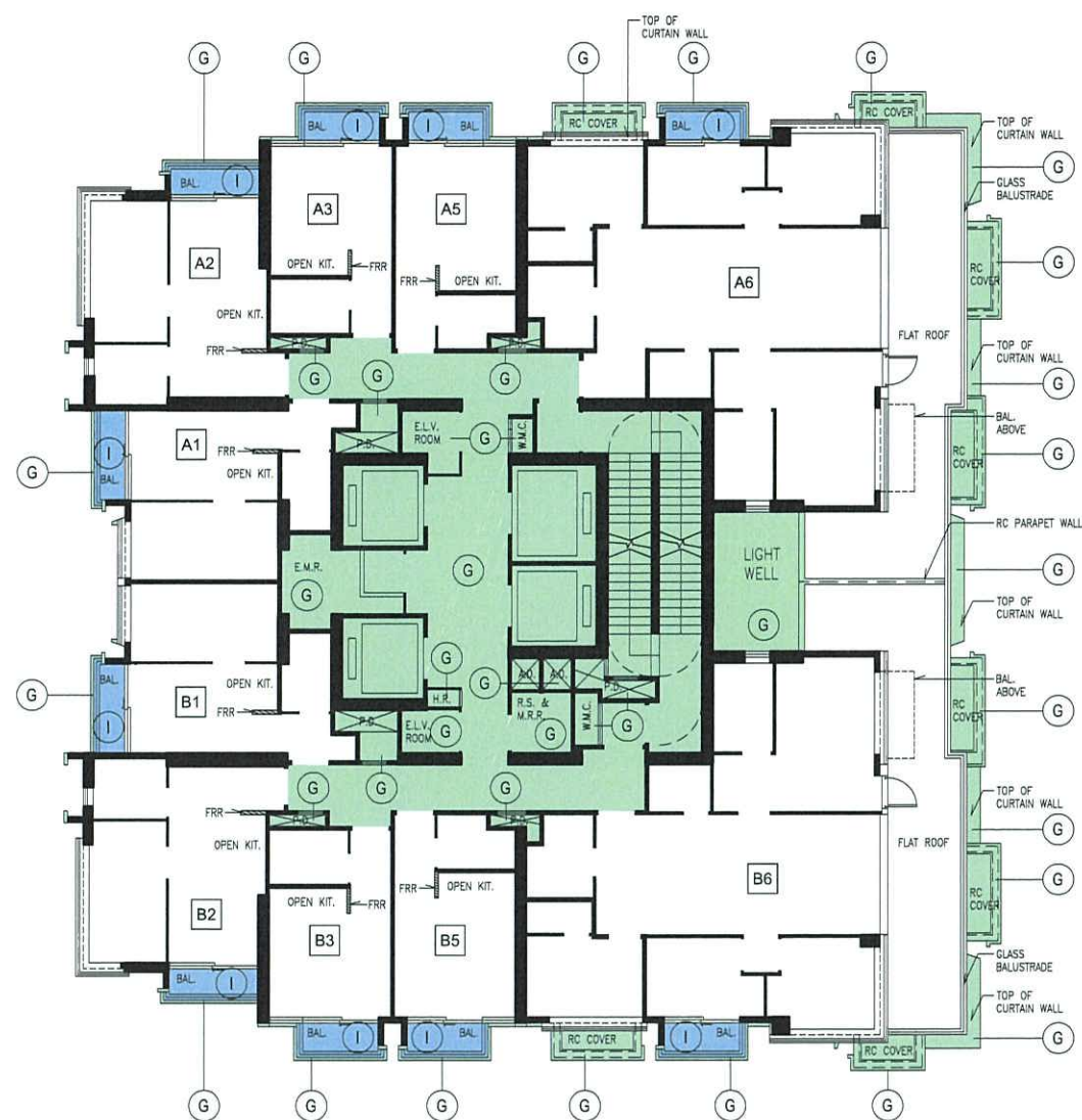
TOWER 1, 37TH FLOOR PLAN
